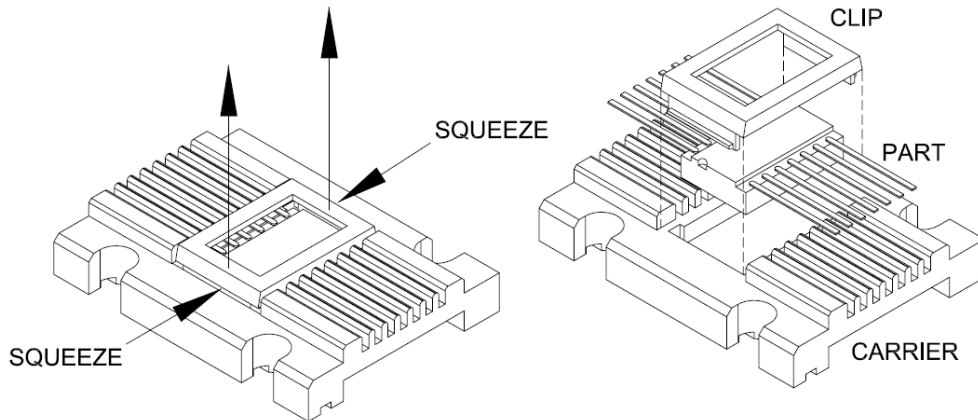
Figure 1 - 14 Lead Flatpack Carrier
