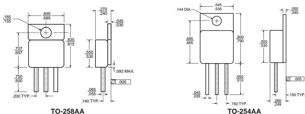
TO-258AA
