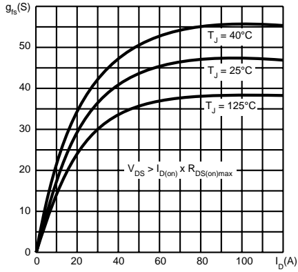
Transconductance
