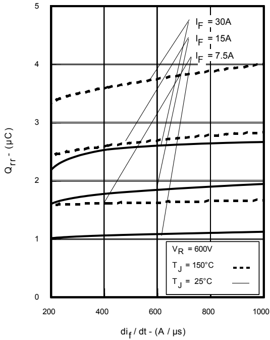
Fig 3. Typical Q_{rr} vs. di/dt
