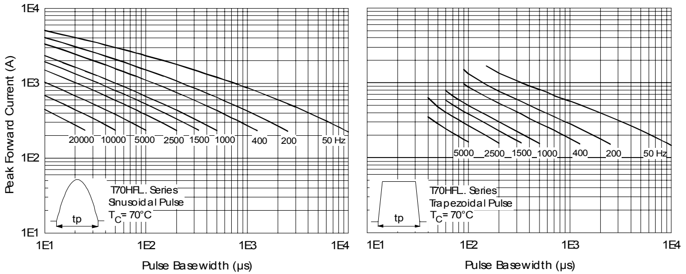
Fig. 40 - Frequency Characteristics
