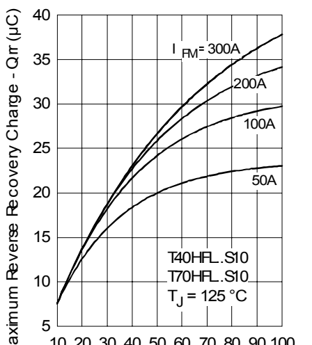
Fig. 26 - Recovery Charge Characteristics
