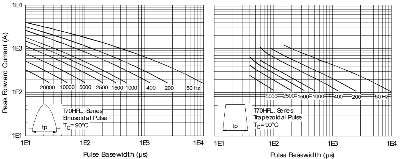
Fig. 41 - Frequency Characteristics
