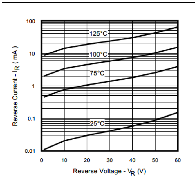
Figure 2 Typical Values of Reverse Current Vs. Reverse Voltage
