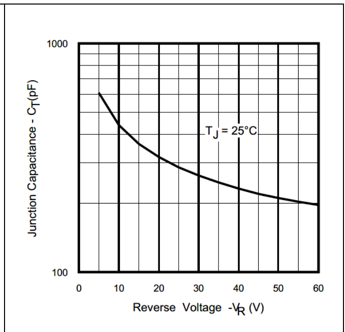
Figure 3 Typical Junction Capacitance Vs. Reverse Voltage
