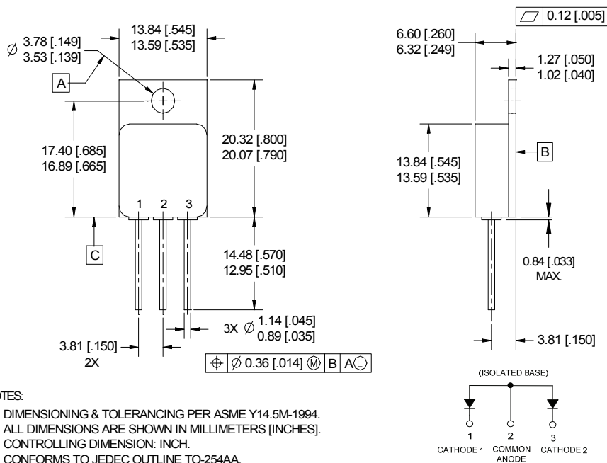
Case Outline and Dimensions - TO-254AA
