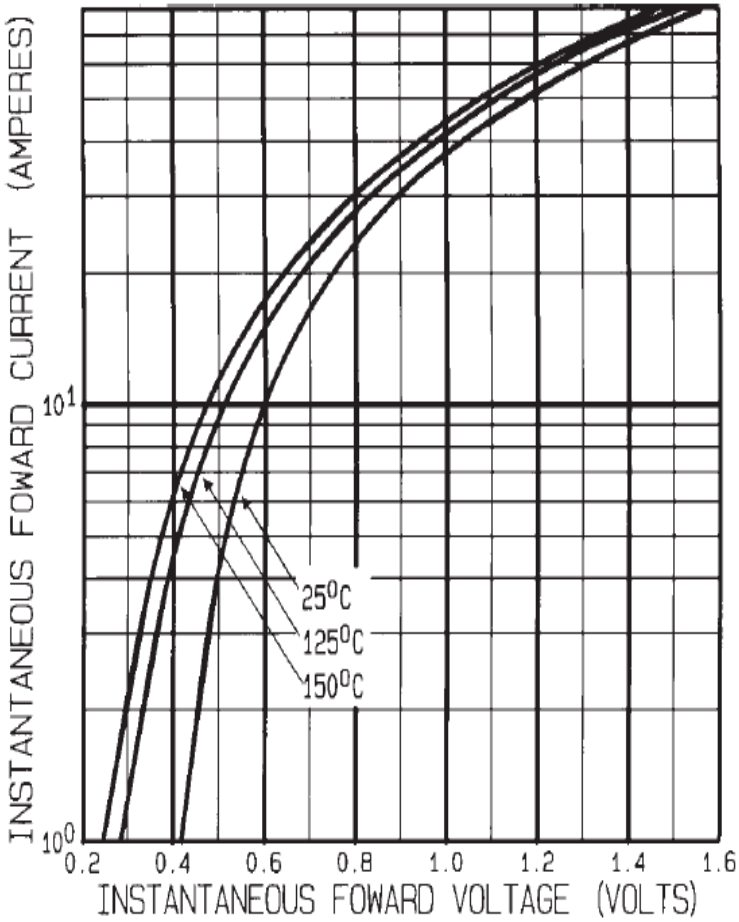
Fig 1. Max. Forward Voltage Drop Characteristics (Per Leg)
