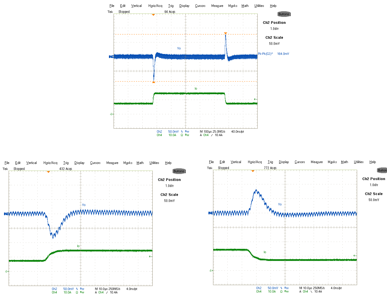
Fig. 13: Transient Response, 7A to 14A step 2.5A/μs Ch 2 :V out , Ch 4 :I out
