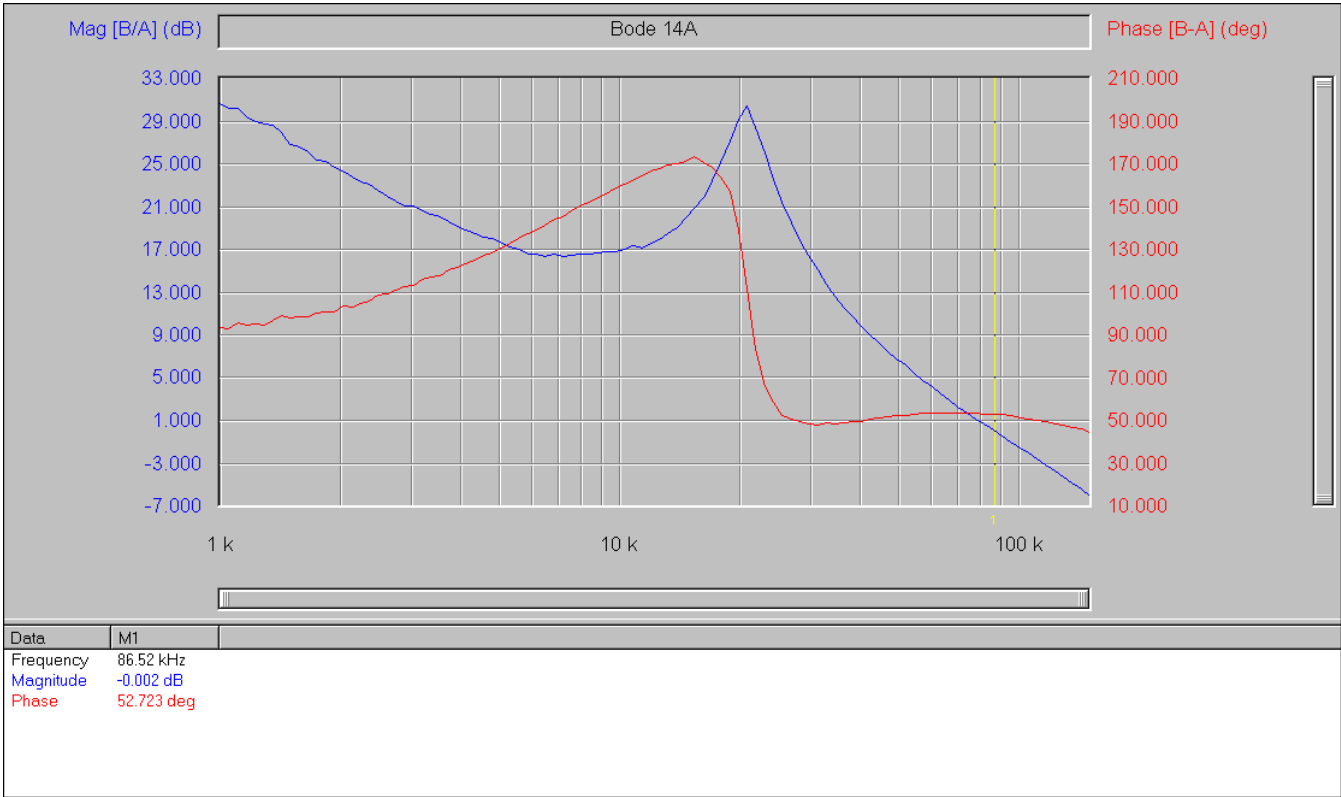
Fig. 14: Bode Plot at 14A load shows a bandwidth of 86kHz and phase margin of 53 degrees
