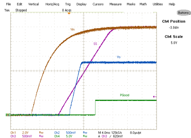
Fig. 8: Start up at 14A Load, Ch 1 :V in , Ch 2 :V o , Ch 3 :V ss , Ch 4 :V PGood
