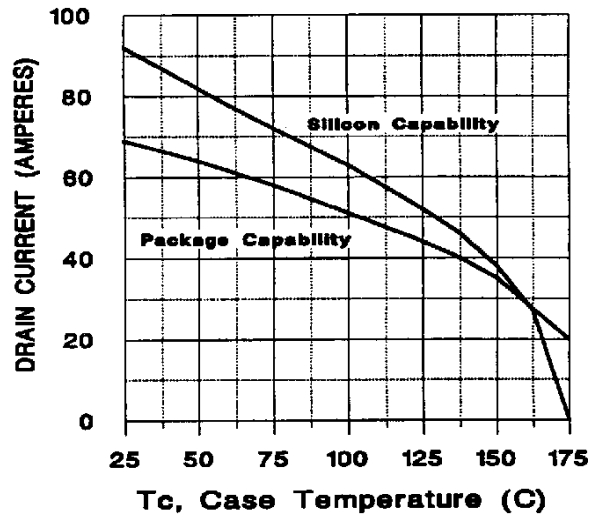
Figure 2 - Current Handling Capability of the TO-220 with a low voltage HEXFET (IRL2203)
