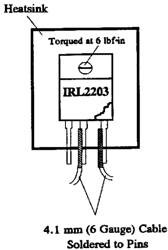
Figure 1 - The Set-Up Used for High Current Tests
