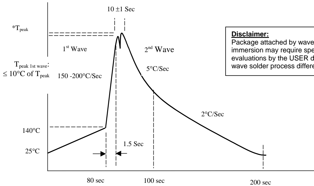
Double Wave Soldering Temperature/Time Profile
