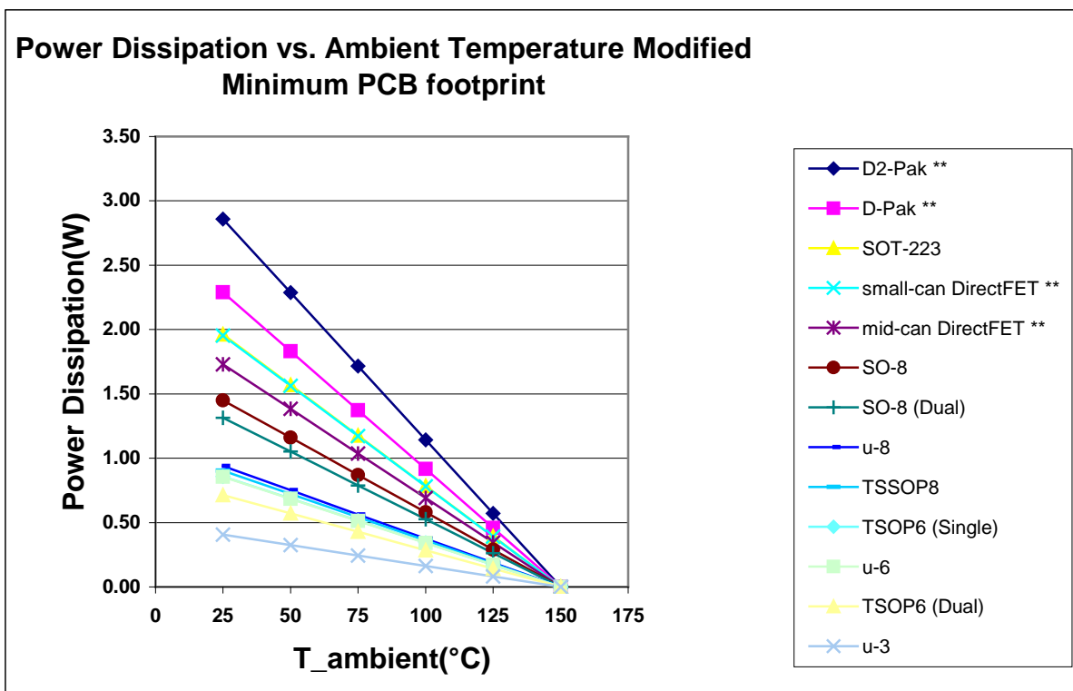
Figure 2: Mod Min Power Dissipation (T_ambient)
