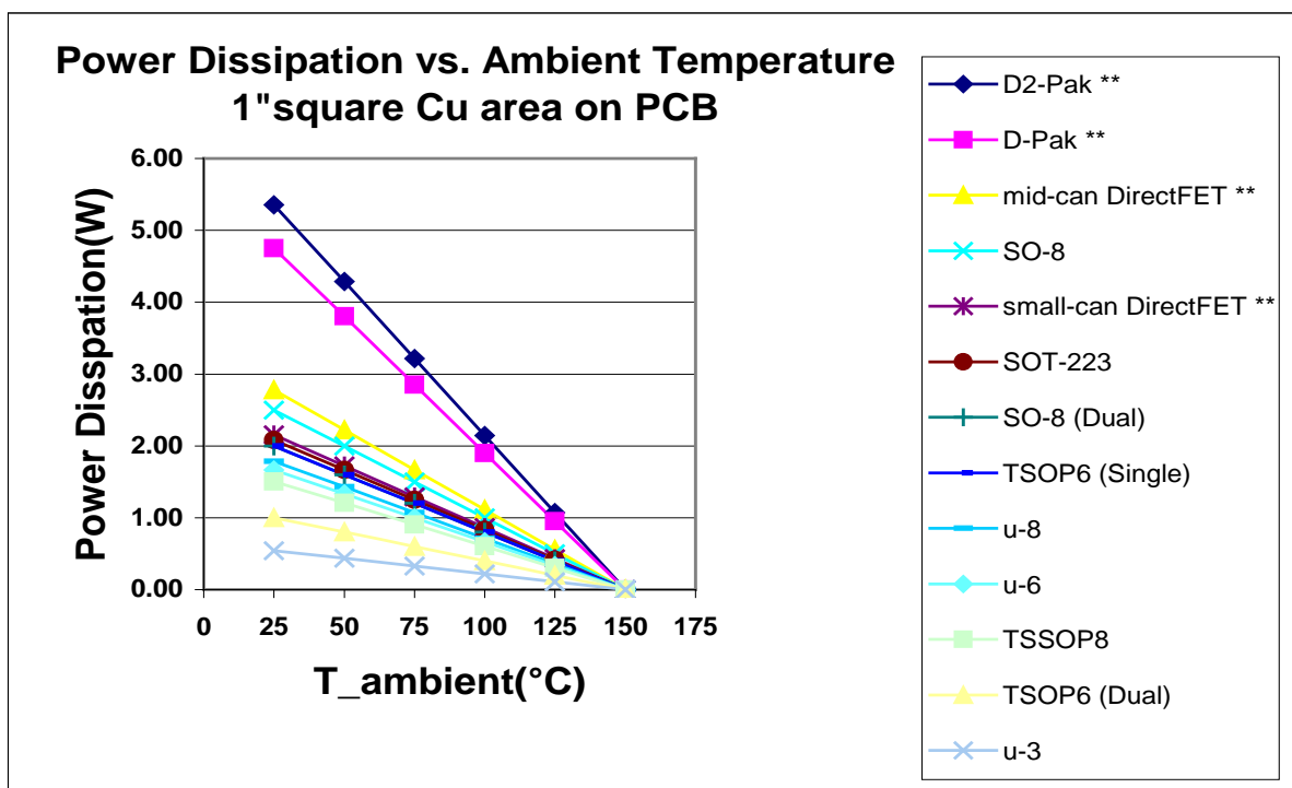
Figure 3: 1 sq" Power Dissipation (T_ambient)
