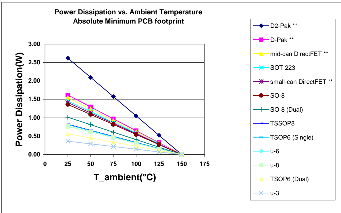
Figure 4: Absolute Min Power Dissipation (T_ambient)
