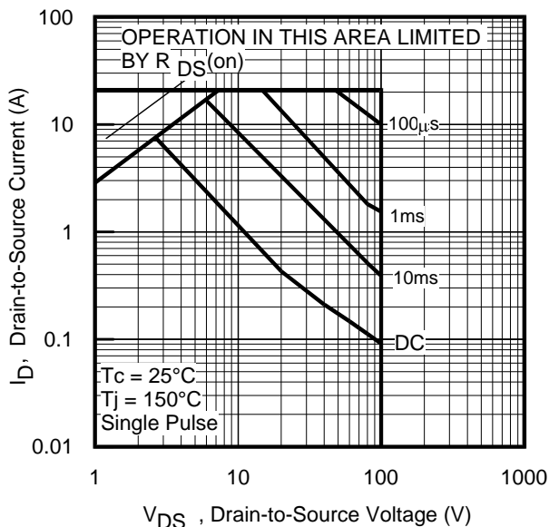
New IRLF120 SOA Curve:
