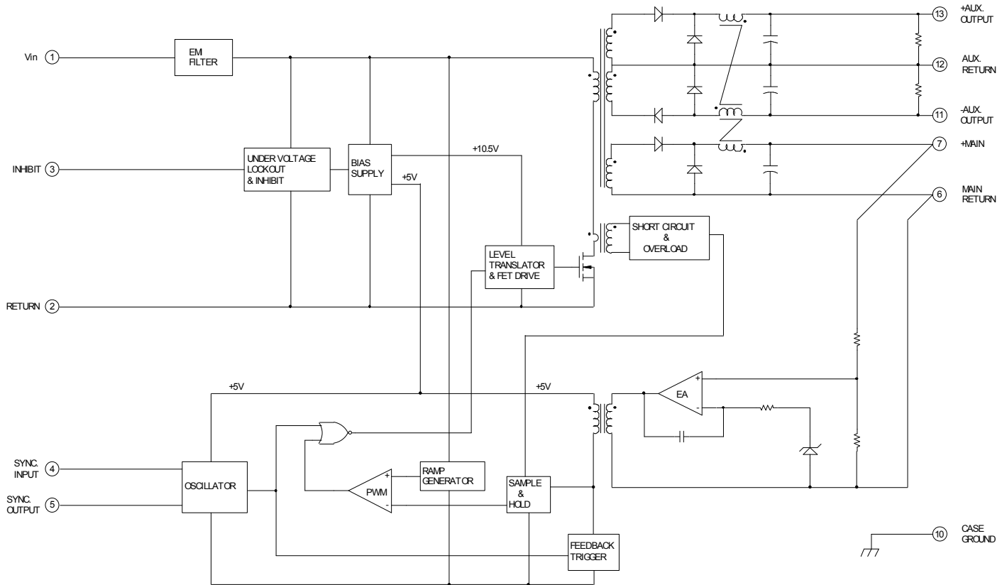
Fig 1. Block Diagram - Triple Output
