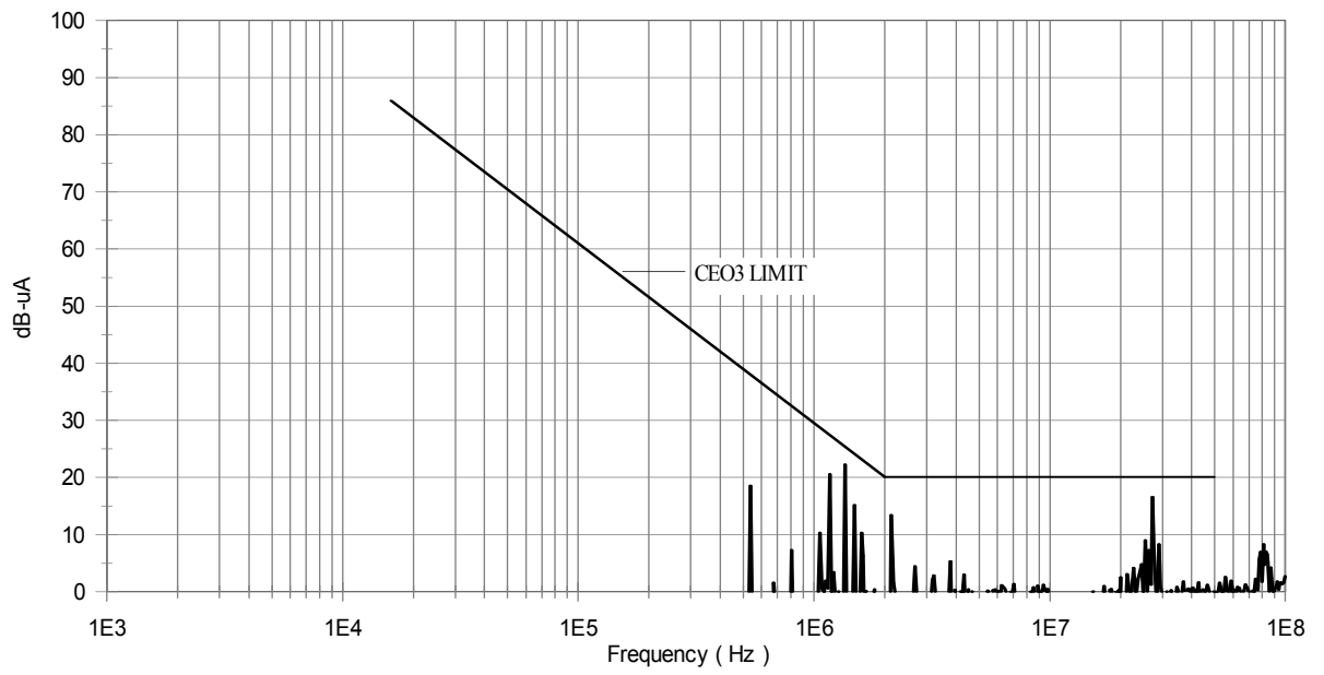
Fig 8. Conducted Emissions, Common Mode
