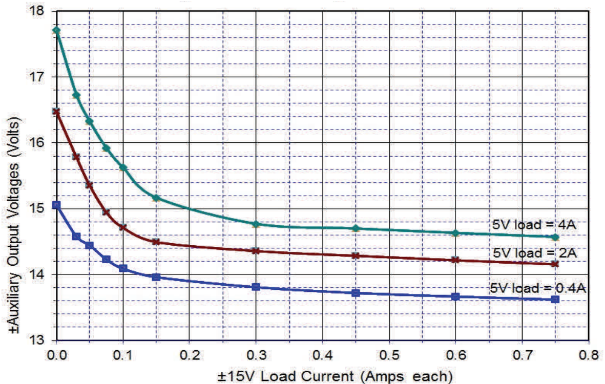
Fig 3. \pm 15V Load Regulation vs 5V Load
