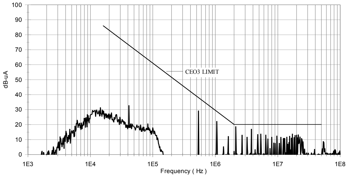
Fig 7. Conducted Emissions, Return Lead
