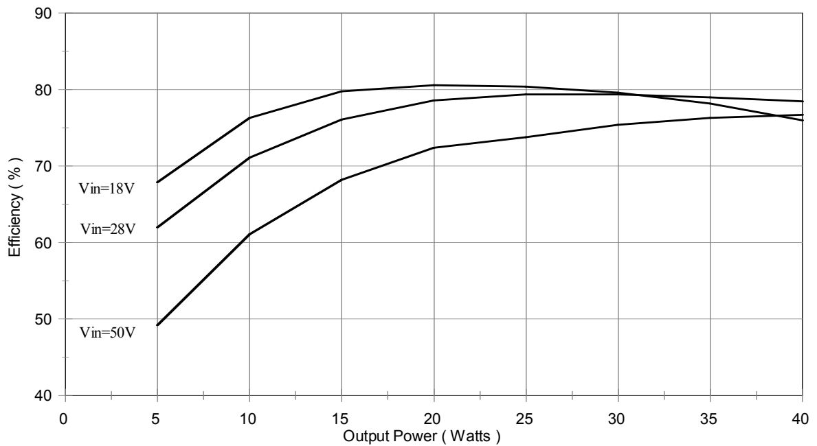
Fig 5. M3G280515T Efficiency vs Line and Load
