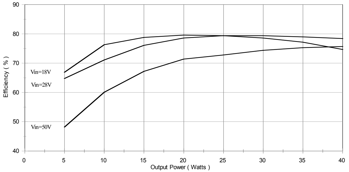
Fig 4. M3G280512T Efficiency vs Line and Load
