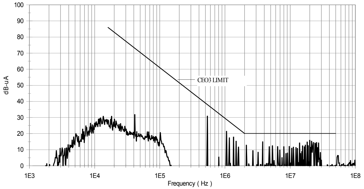
Fig 6. Conducted Emissions, Positive Lead
