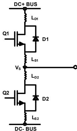
Figure 9: Parasitic Elements
