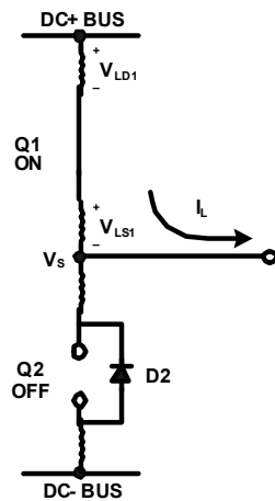
Figure 10: V_S positive
