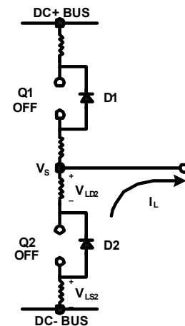
Figure 11: V_S negative
