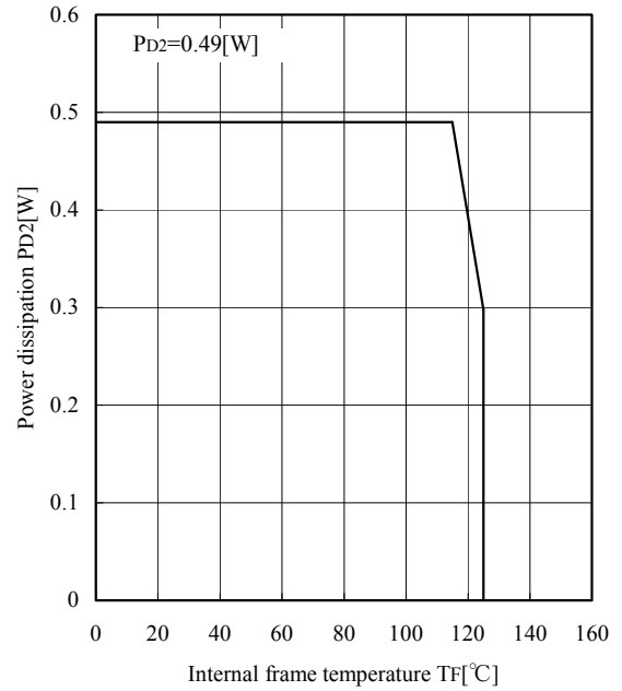
IRIS-F6428S MIC TF-PD2 Curve
