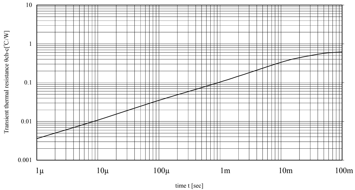
IRIS-F6428S Transient thermal resistance curve
