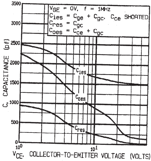
Fig. 7 - Typical Capacitance vs. Collector-to-Emitter Voltage
