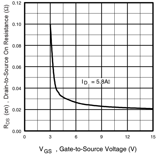
Fig 6. Typical On-Resistance Vs. Gate Voltage
