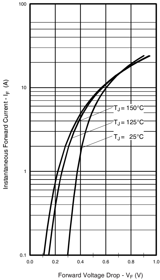
Fig. 11 - Typical Forward Voltage Drop Characteristics
