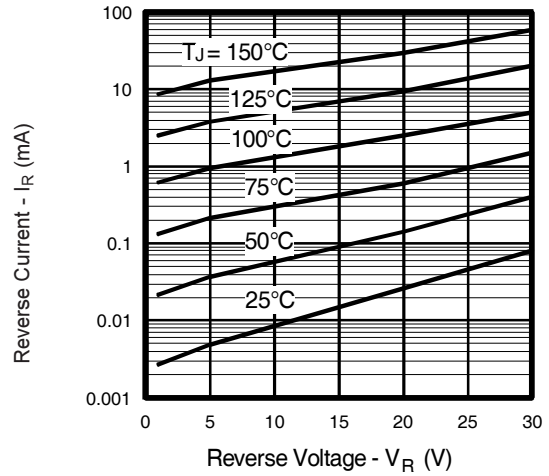
Fig. 12 - Typical Values of Reverse Current Vs. Reverse Voltage
