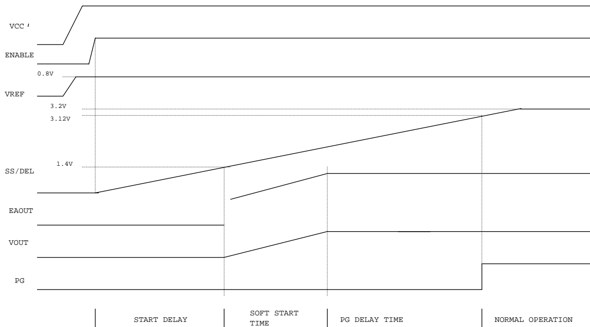
Figure 8 - Start-up sequence
