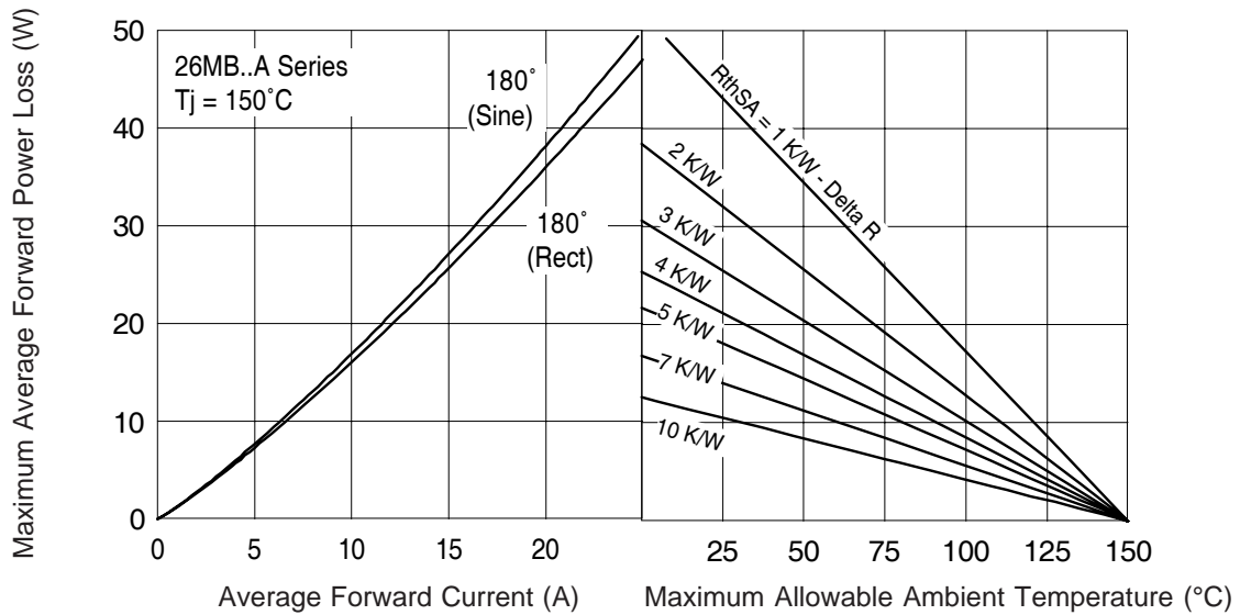
Fig. 3 - Total Power Loss Characteristics
