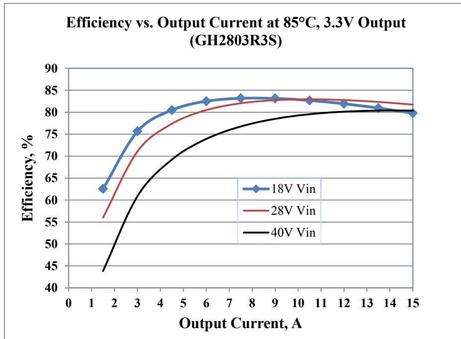
Figure 19 – Typical Efficiency Performance vs. Output Load and Input Voltage At +85°C, GH2803R3S (3.3V/15A Output)
