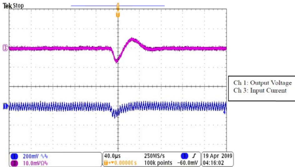
Figure 12 – Output Fluctuation under SEE, 60MeV·cm 2 /mg, Vin = 18V, S/N 005
