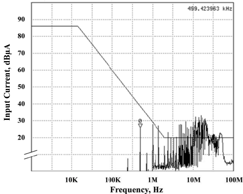
Figure 6 - Conducted Emission, Common Mode
