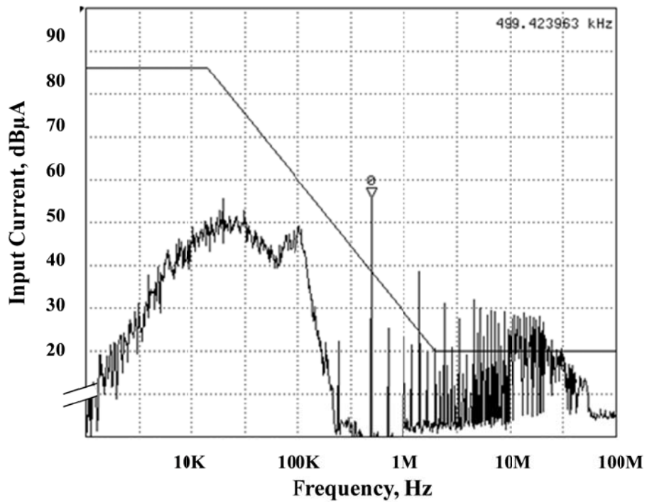
Figure 8 - Conducted Emissions, Differential, Return Line
