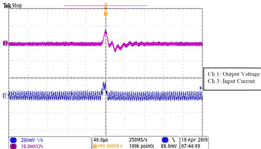
Figure 14 – Output Fluctuation under SEE, 86.9MeV·cm 2 /mg, Vin = 28V, S/N 004
