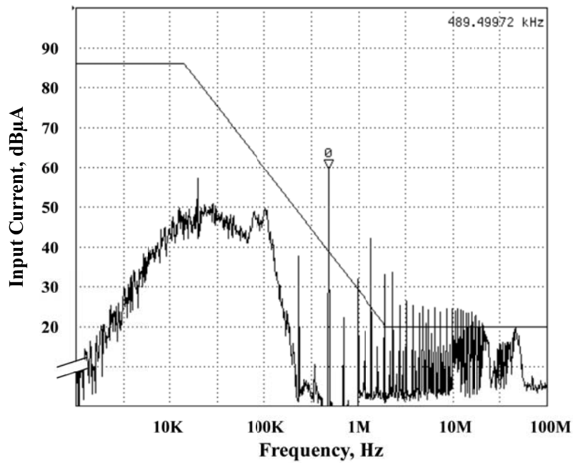
Figure 7 - Conducted Emissions, Differential, Positive Line
