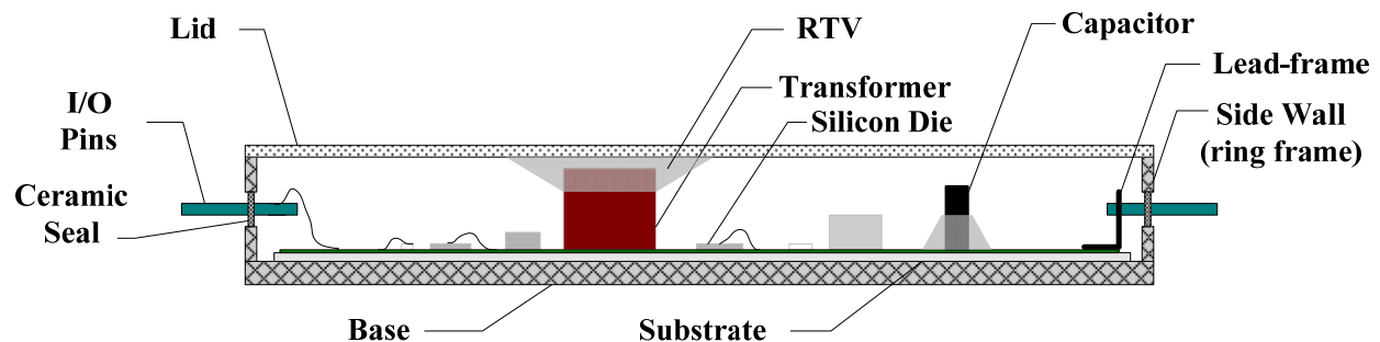
Figure 10 – A Simplified Cross Sectional View of a GH Hybrid Converter Assembly
