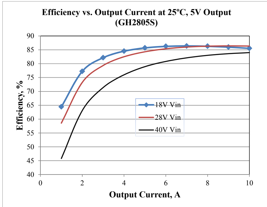
Figure 20 – Typical Efficiency Performance vs. Output Load and Input Voltage At +25°C, GH2805S (5V/10A Output)
