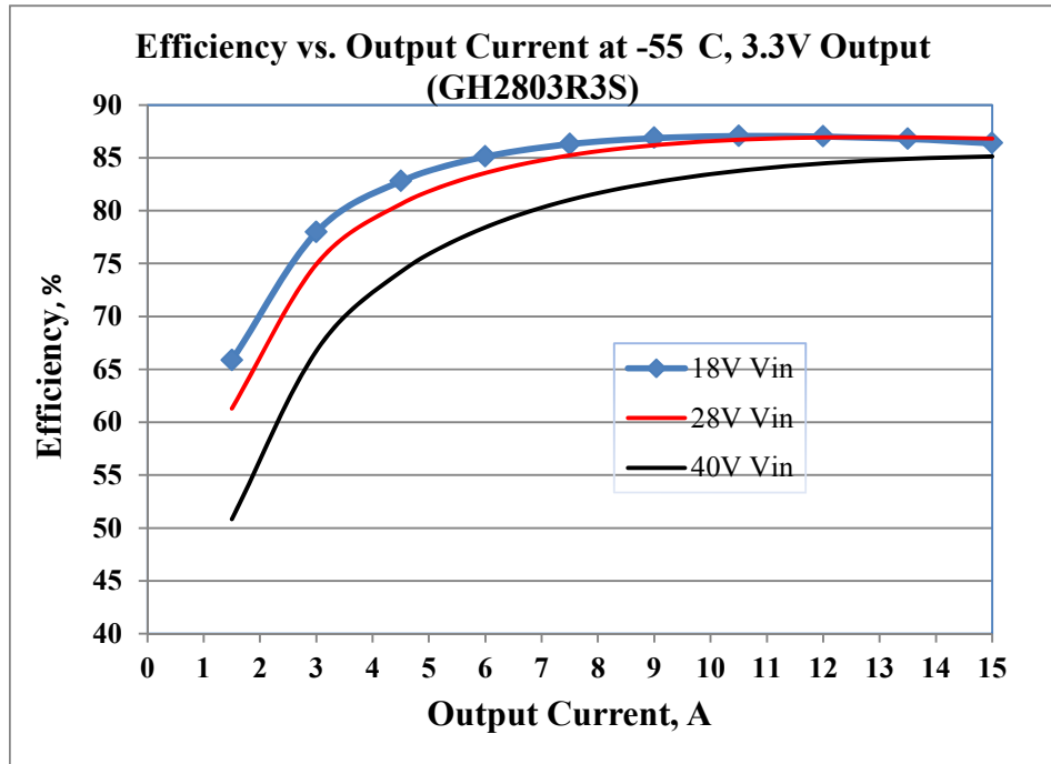
Figure 18 – Typical Efficiency Performance vs. Output Load and Input Voltage At -55°C, GH2803R3S (3.3V/15A Output)
