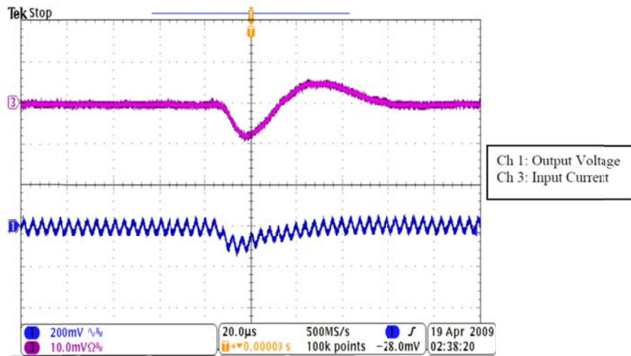
Figure 11 – Output Fluctuation under SEE, 37MeV·cm 2 /mg, Vin = 18V, S/N 005
