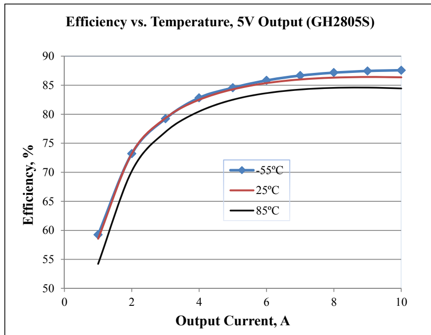
Figure 21 – Typical Efficiency Performance vs. Temperature and at Nominal Input Voltage, GH2805S (5V/10A Output)
