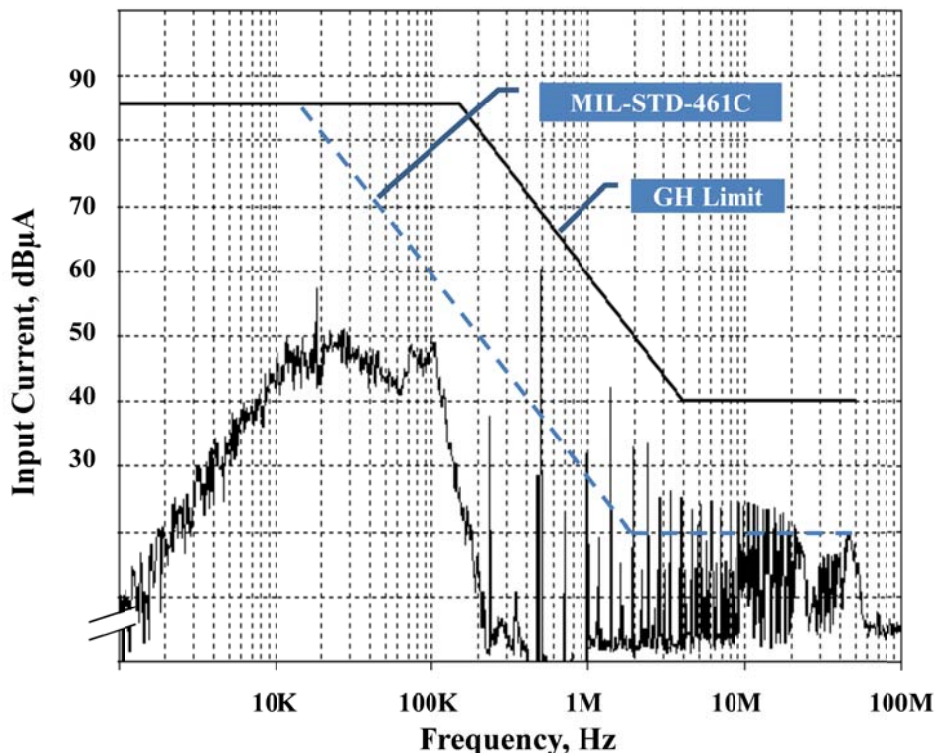
Figure 9 — Conducted Emission, Differential Mode, Positive Line with GH CE03 and MIL-STD-461C Limits
