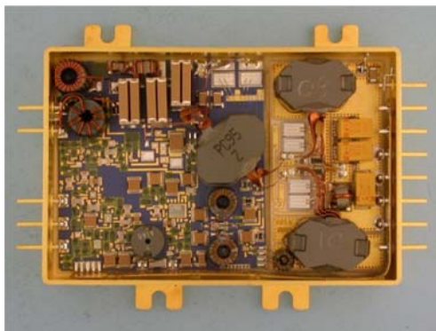
Figure 3- Internal View of a GH Converter Figure 4 – External View of a GH Converter
