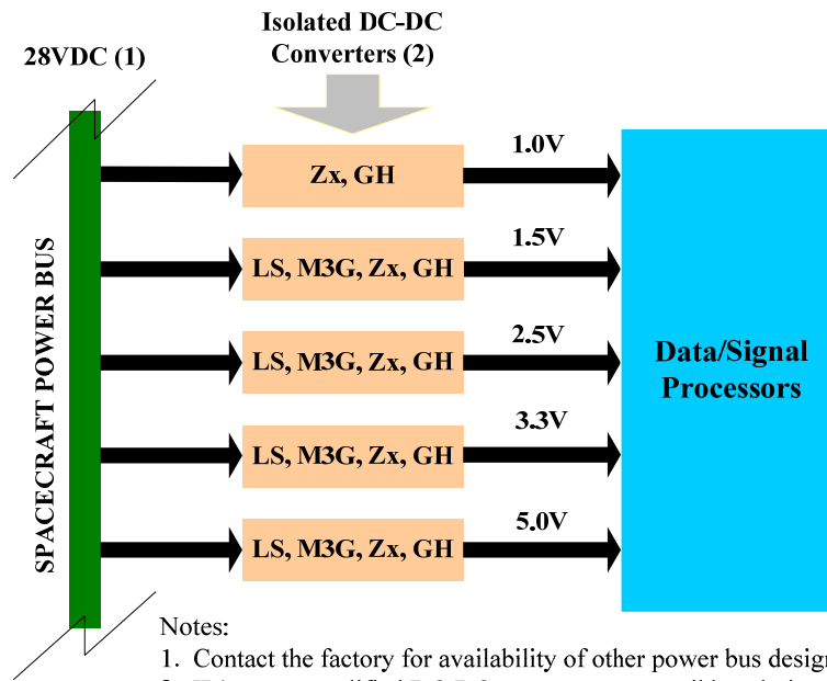
Figure 2 – A simplified De-centralized Power System Diagram
