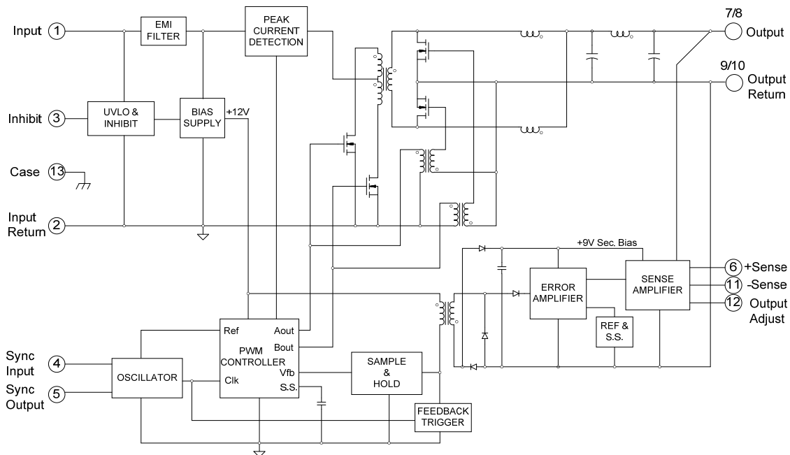
Figure 5 - GH Series Block Diagram
