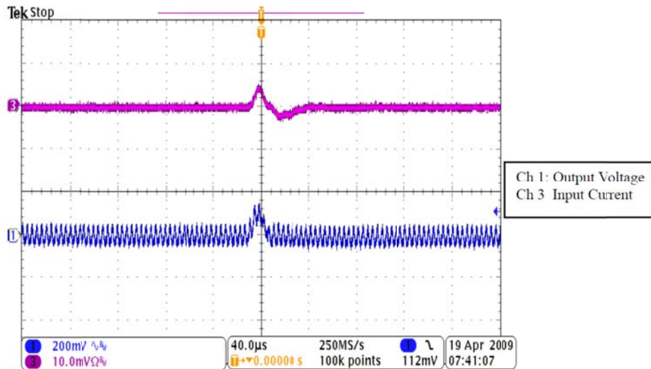
Figure 13 – Output Fluctuation under SEE, 86.9MeV·cm 2 /mg, Vin = 50V, S/N
