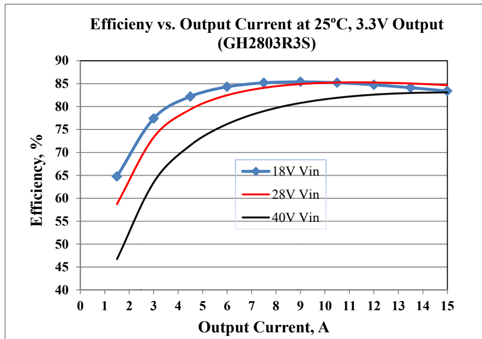
Figure 17 – Typical Efficiency Performance vs. Output Load and Input Voltage At +25°C, GH2803R3S (3.3V/15A Output)
