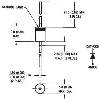
Outline DO-201AD
