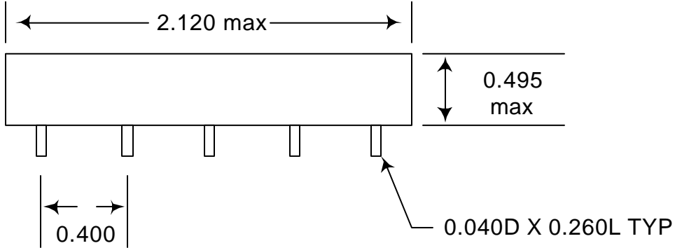
Case Style AHE (unflanged)
