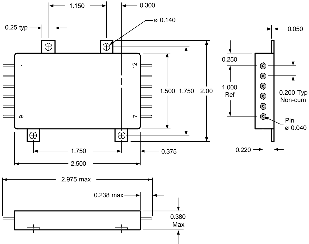
Case Style AFL/AME/AHP (Type Y)
