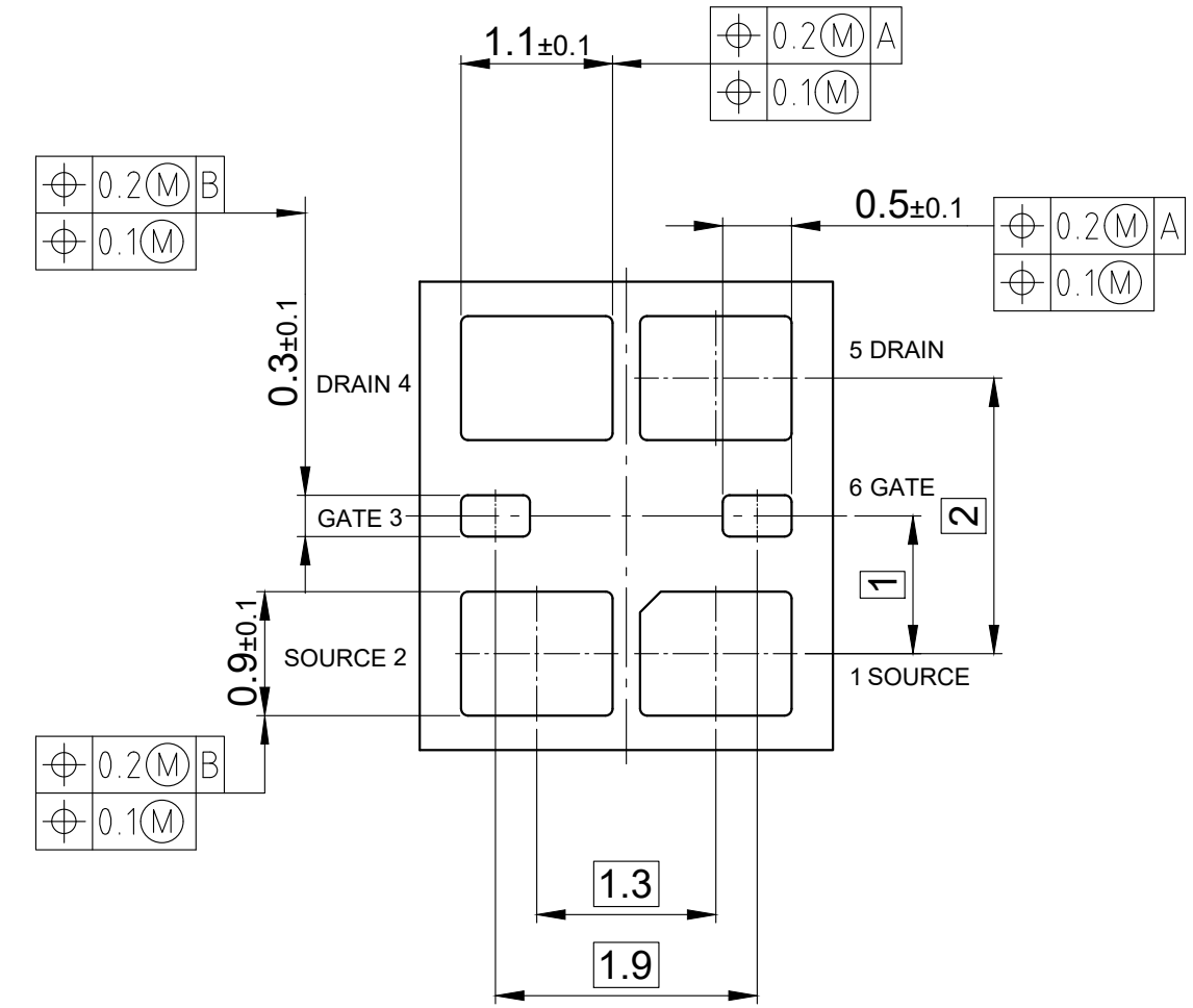
Bottom view
