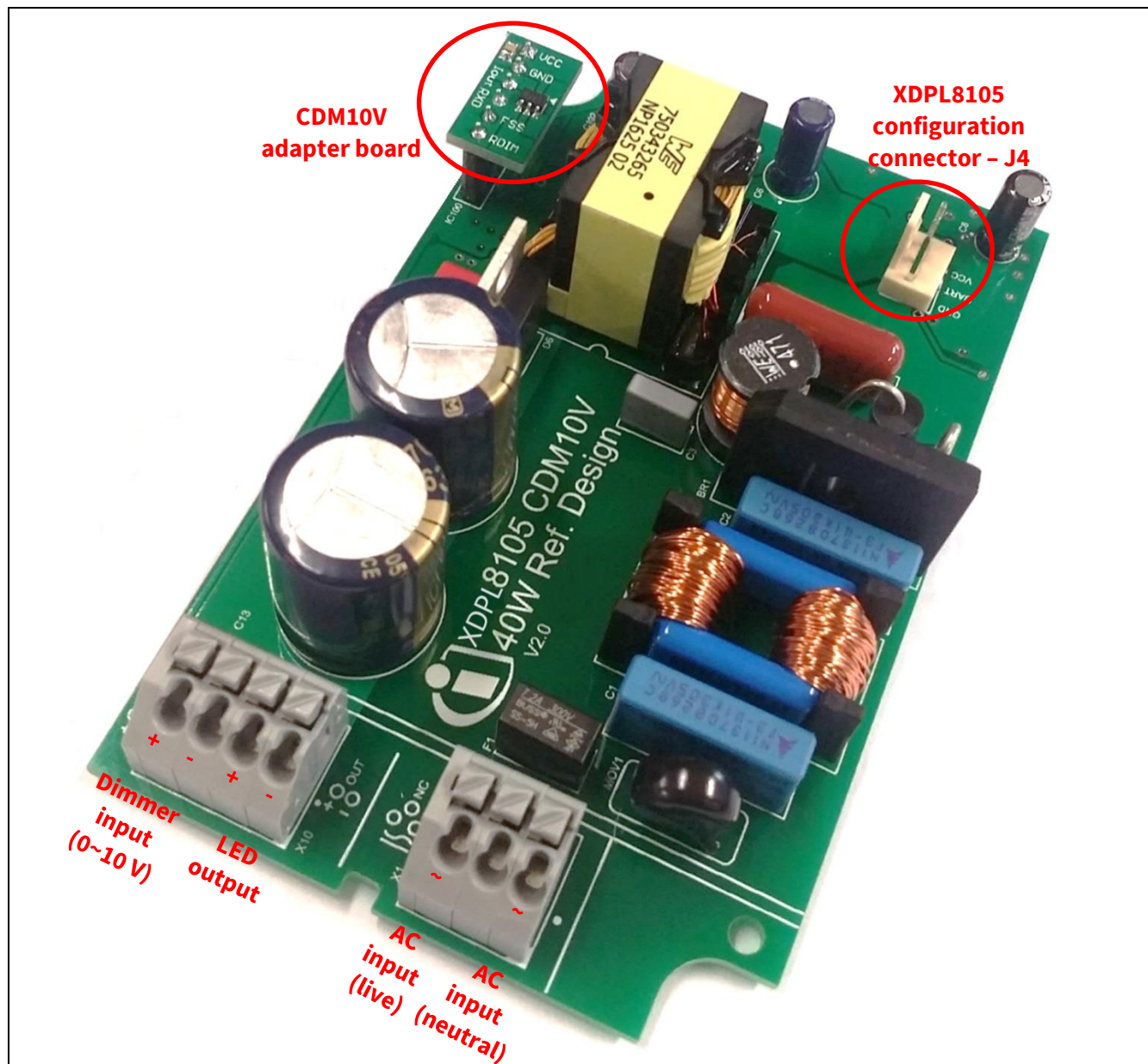
Figure 1 XDPL8105 40 W reference design with CDM10V adapter board and configuration connector
