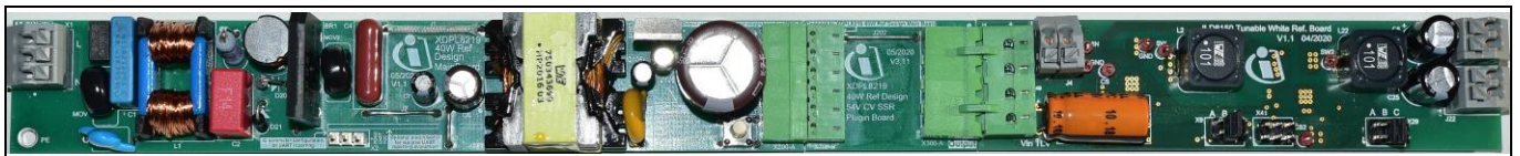
Figure 3 Modular concept – primary stage, constant voltage feedback, ILD8150E tunable white
