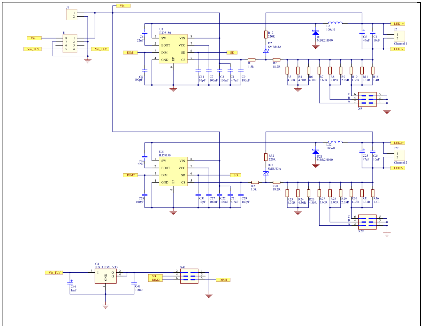
Figure 4 ILD8150E tunable white evaluation board circuit
